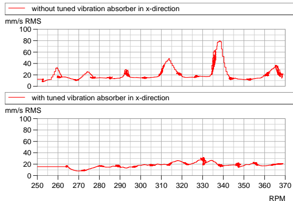
Figure 11: Measured pipeline vibrations with and without the tuned absorber in x-direction
