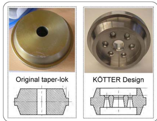
Figure 20: Original and modified taper-lok-plates
