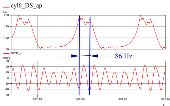
Figure 18: Trend of internal cylinder pressure (head end) and vibration velocity at measuring point MP31
