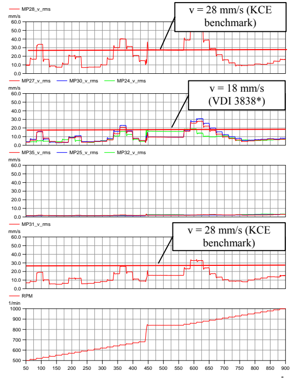
Figure 15: RMS-vibration velocities (z-direction) and guideline at the 2 nd stage of the compressor as well as the RPM (*VDI: Verein Deutscher Ingenieur: Association of German Engineers)
