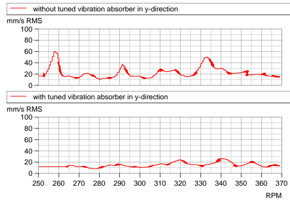
Figure 12: Measured pipeline vibrations with and without the tuned absorber in y-direction
